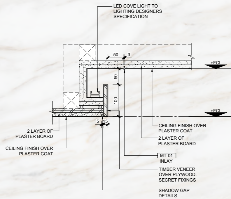
TYPICAL CEILING DETAIL 2
