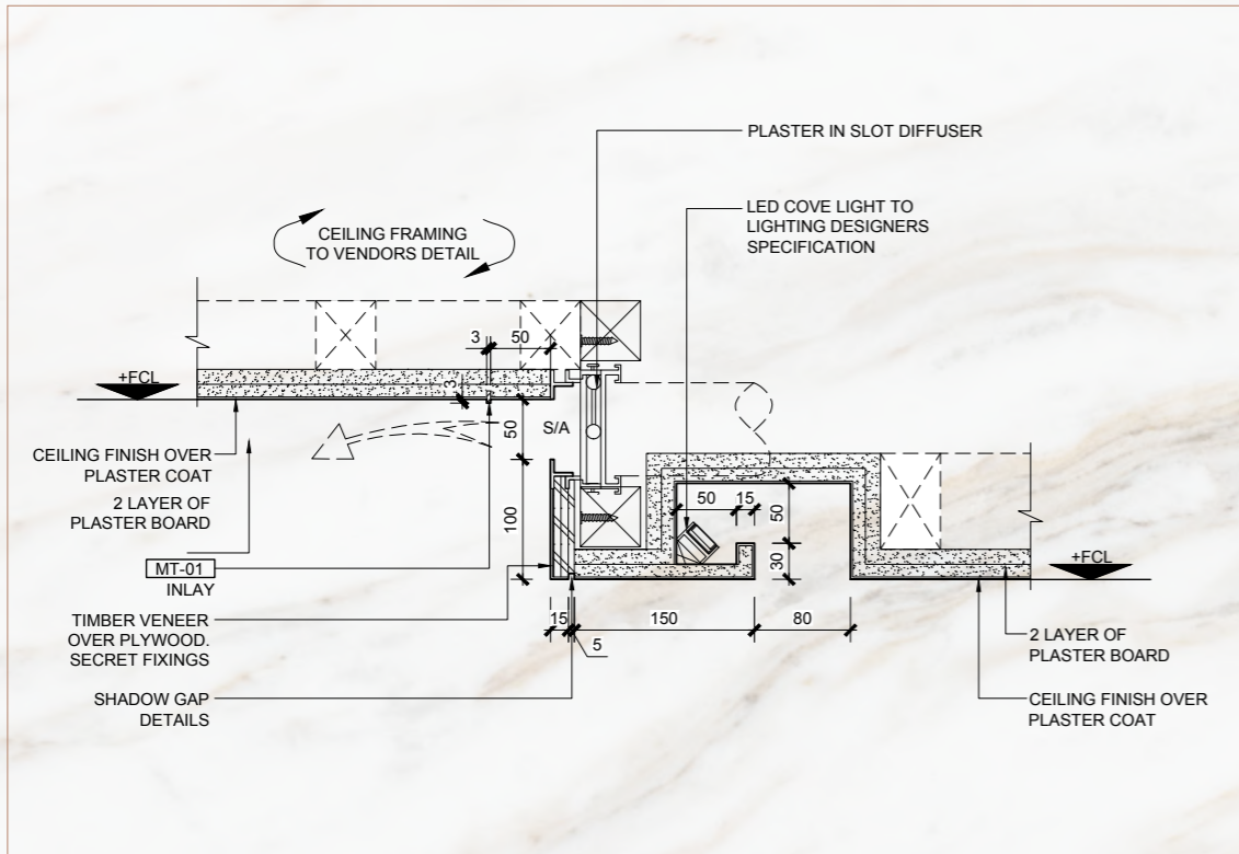
TYPICAL CEILING DETAIL 1
